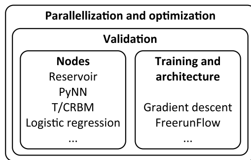
Figure 1: A schematic overview of the structure of Oger. The basic processing blocks (nodes) are combined with methods for constructing and training architectures. These architectures can then be evaluated in a validation and optimization framework.
