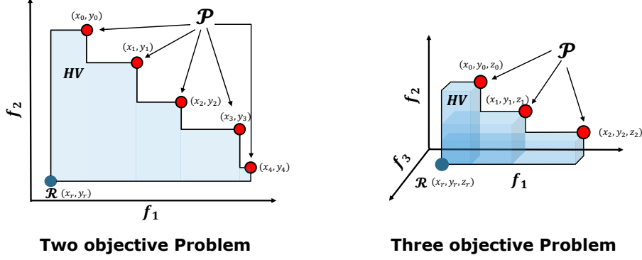
Figure 4: Visualization of example hypervolume calculation.
