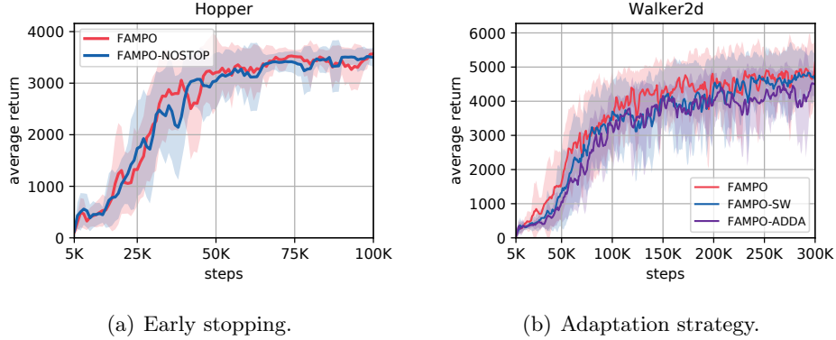
Figure 9: More empirical analysis for FAMPO. (a) FAMPO-NOSTOP denotes the FAMPO variant without early stopping the model adaptation procedure. (b) FAMPO-SW denotes the FAMPO variant of sharing the feature extractor weights for two data distributions. FAMPO-ADDA denotes the FAMPO variant of fixing the feature extractor of real data.
