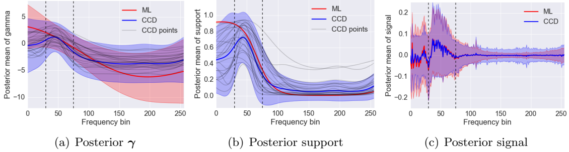
Figure 9: Comparison of the posterior distribution of \gamma , \mathbf{z} and \mathbf{x} for ML and CCD hyper-parameter inference. The posterior distribution for the CCD approximation is a mixture model and the thin black solid lines show the posterior mean of each individual component. These are omitted for the posterior of the signal to improve visual clarity.
