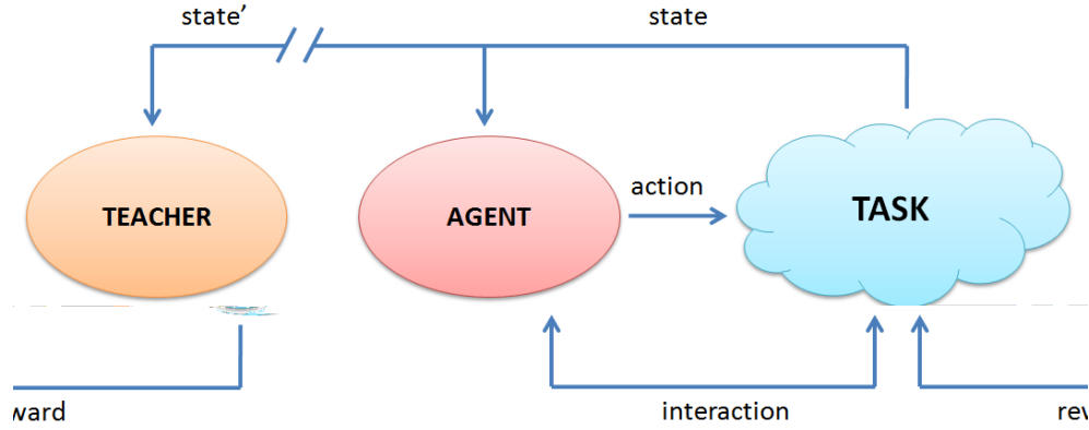
Figure 3: General Teacher-Learner Agent Interaction Scheme.
