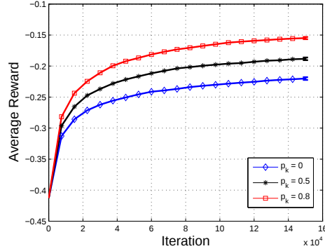
Figure 3: Policy Gradient with a Partial Model. Implementation of the algorithm described in Section 6.2 on a GARNET(30,5,10,1) MDP, with step size parameters \varepsilon = 0.03 and \varepsilon' = 0.003 . The linear FA parameters are L = 10 and l = 2 . Average reward is plotted vs. iteration number for different values of p_k . Results are averaged over 500 different runs with the same initial conditions. Error bars display the standard error of the mean; for clarity of presentation the bars are displayed only for the last iteration.
