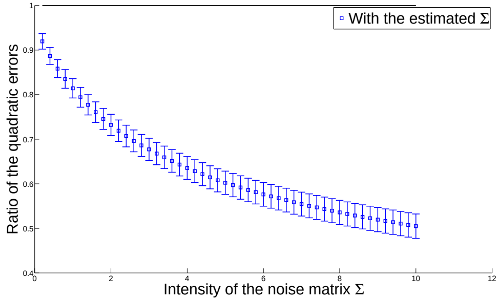
Figure 8: Increasing the signal-to-noise ratio (Experiment C), improvement of multi-task compared to single-task: \mathbb{E}[\|\hat{f}_{\text{similar},\hat{\Sigma}} - f\|^2 / \|\hat{f}_{\text{ind},\hat{\Sigma}} - f\|^2] .
