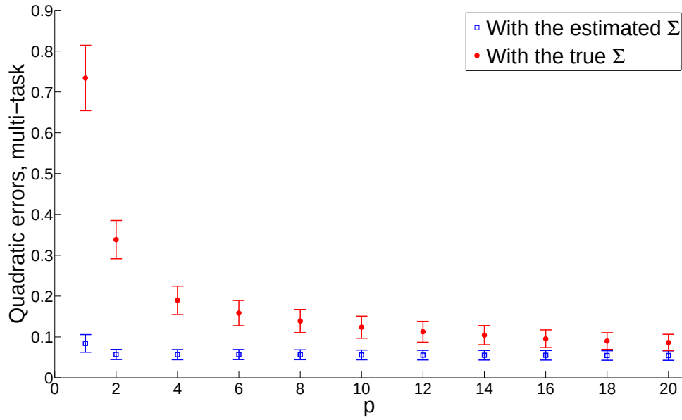
Figure 2: Increasing the number of tasks p (Experiment A), quadratic errors of multi-task estimators (np)^{-1}\mathbb{E}[\|\hat{f}_{\text{similar}, S} - f\|^2] . Blue: S = \hat{\Sigma} . Red: S = \Sigma .
