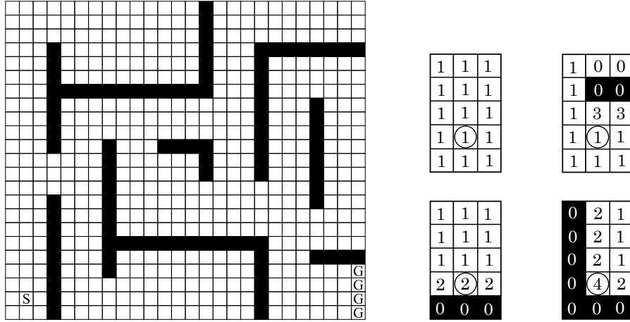
Figure 12: Left, the large maze task, in which the agent must travel from S to one of the G’s. Right, transition probabilities ( \cdot \frac{1}{15} ) of a ‘north’ action for different positions of the agent (indicated by the circle) with respect to the walls (black squares). When the transition to a square is blocked by a wall, its transition probability is added to that of the square in front of the wall.
