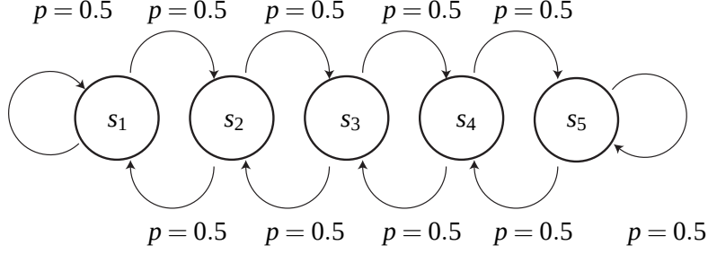
Figure 3: A five-states MRP.
