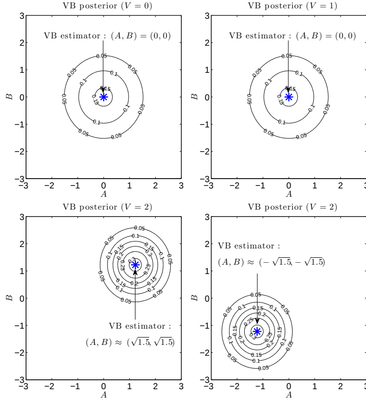
Figure 6: VB posteriors and VB solutions when L = M = 1 (i.e., the matrices V , U , A , and B are scalars). When V = 2 , VB gives either one of the two solutions shown in the bottom row.
