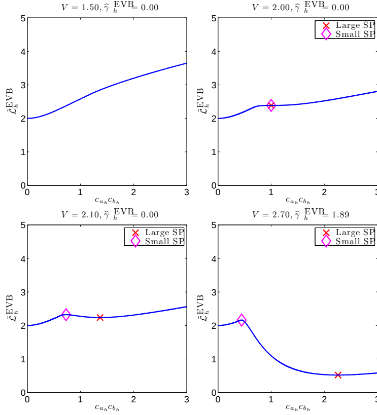
Figure 13: Illustration of the partially minimized objective function (175) when L = M = H = 1 , \sigma^2 = 1 , and V = 1.5, 2.0, 2.1, 2.7 . The convergence \tilde{\mathcal{L}}_h^{\text{EVB}}(c_{a_h}c_{b_h}) \rightarrow L + M (= 2) as c_{a_h}c_{b_h} \rightarrow 0 is observed (see Equation (176)). 'Large SP' and 'Small SP' indicate the large and the small positive stationary points, respectively.
