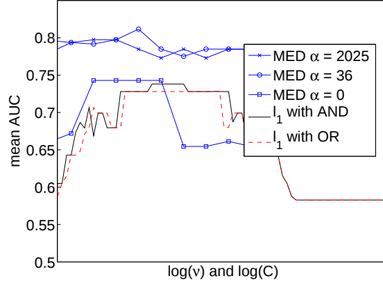
Figure 4: Graphical model structure estimation from data sampled from Ising models. The average area under the curve is shown for ten random models. The proposed method is evaluated across various values of C and \alpha and compared to \ell_1 regularized logistic regression method across various values of v with both AND and OR symmetrization.
