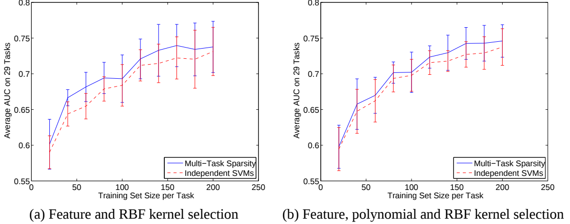
Figure 2: Feature selection and kernel selection on the Landmine data set. In (a), feature selection is combined with RBF kernel selection. In (b), feature selection is combined with both polynomial and RBF kernel selection. Multitask sparse kernel selection and independent SVM classification are compared. Various data set sizes are shown ranging from 20 to 200 samples for each of the 29 tasks. The average area under the ROC curve on test data is shown for all tasks for 5 folds (along with the standard deviation). The values of C and \alpha were obtained by cross-validation on held out data.
