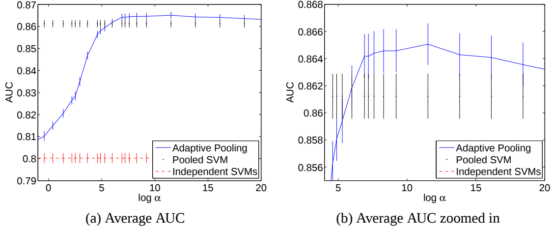
Figure 3: Adaptive pooling experiments on the Heart data set. The area under the curve (AUC) for adaptive pooling, pooling and independent SVMs is shown in (a). In (b), a zoomed in version of the plot is shown to focus on the setting with highest average AUC. The value of the regularization parameter C was found using cross-validation for all three methods.
