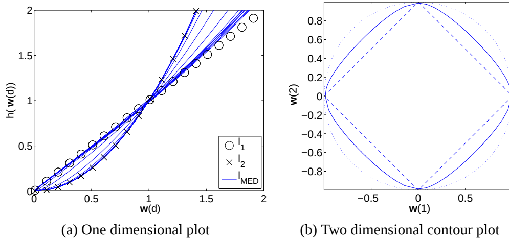
Figure 6: Various penalties on the classifier weights. In (a), the penalties are shown as one dimensional functions of the form h(\mathbf{w}(d)) as \alpha varies from \alpha = 0 (which mimics an \ell_2 norm) to large \alpha large (which resembles an \ell_1 norm). In (b), a two-dimensional contour plot is provided showing the shape of the \ell_1 penalty as a dashed line, the shape of the \ell_2 penalty as a dotted line and the shape of the \ell_{MED} penalty with \alpha = 2 as a solid line.
