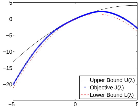
Figure 5: Upper and lower quadratic bounds on the objective function.
