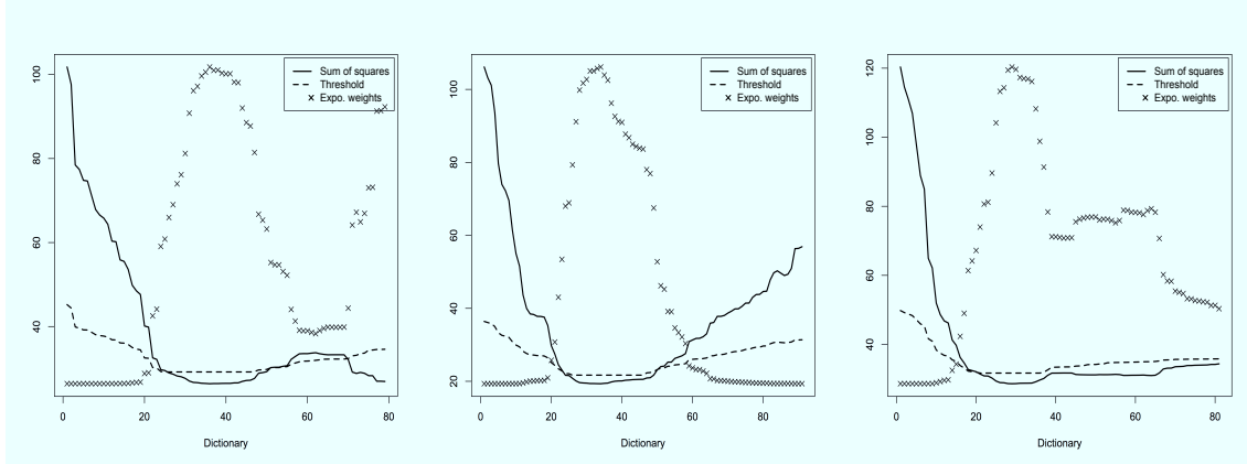
Figure 2: Empirical risk R_{n,1}(f) , value of the threshold R_{n,1}(\hat{f}_{n,1}) + 2\max(\phi\|\hat{f}_{n,1} - f\|_{n,1}, \phi^2) and weights of the AEW (rescaled) for f \in F , where F is a dictionary obtained using LARS, see Section 3 below. Only the elements of F with an empirical risk smaller than the threshold are kept from the dictionary for the construction of the aggregates of Definition (1). The first and third examples correspond to a case where an aggregate with preselection step improves upon AEW, while in the second example, both procedures behaves similarly.
